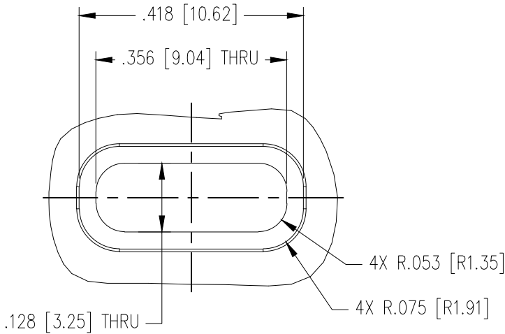
REAR VIEW: PANEL CUT-OUT
