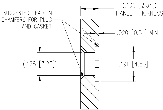
SIDE SECTION VIEW: PANEL CUT-OUT
