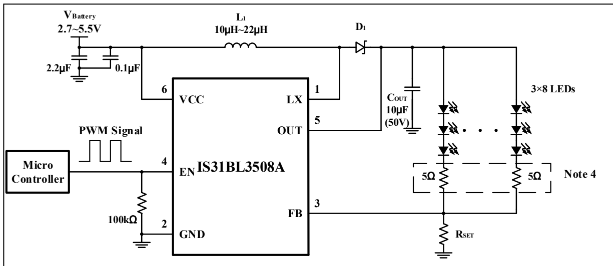
Figure 3 Constant Current White LED Driver Using PWM At The EN Pin To Control Intensity 3 x 8 LEDs
