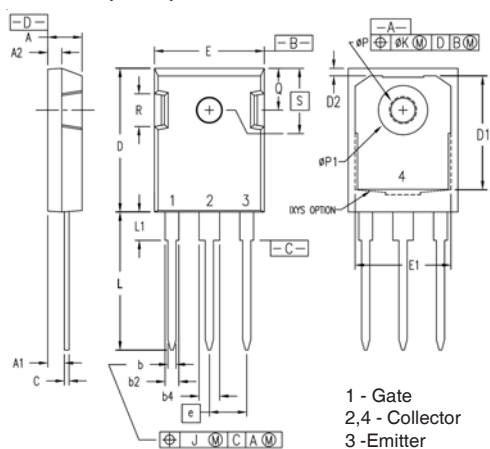
TO-247 (IXYH) Outline
