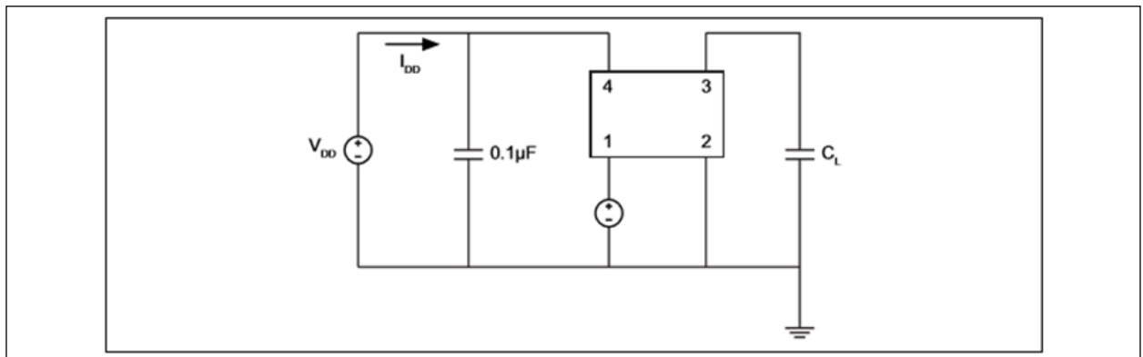
FIGURE 5-1: Test Circuit.
