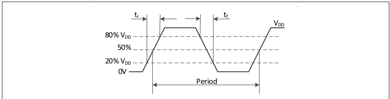
FIGURE 4-1: Output Waveform.
