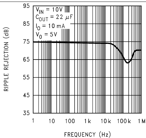
Figure 9. Ripple Rejection
