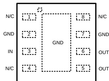
WSN (NGN) Package 8 Pins Top View
