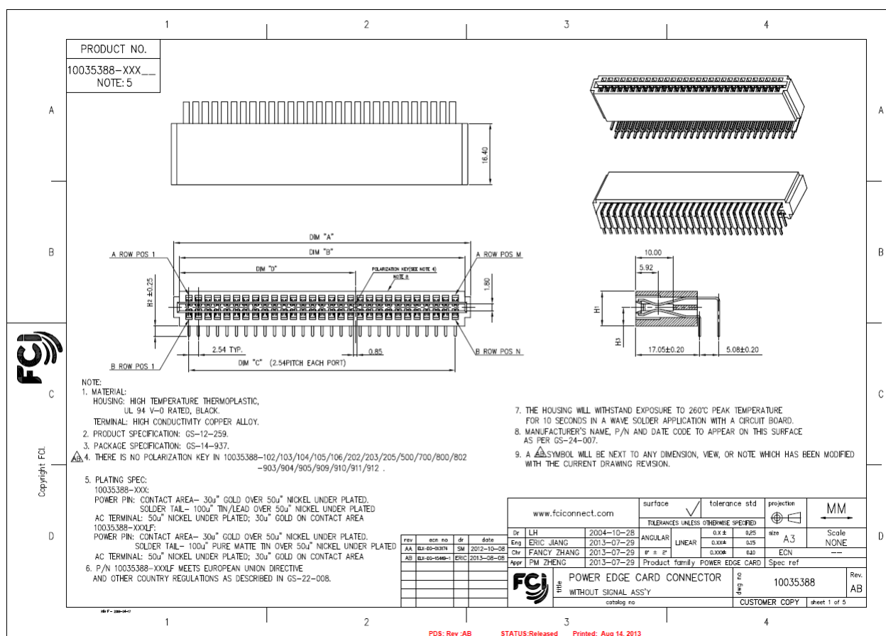
Figure 27. Mating connector drawing page 1
