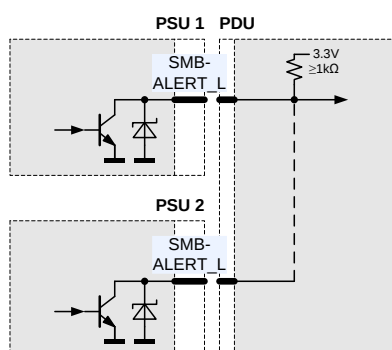
Figure 15. SMBALERT_L connection
