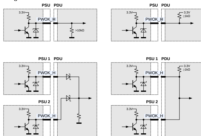
Figure 7. PWOK_H connection
