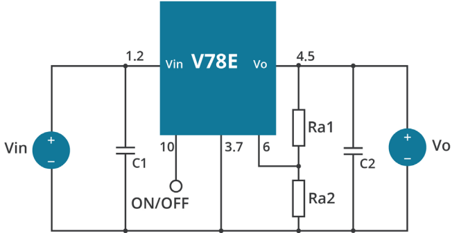
Figure 1 Application Circuit
