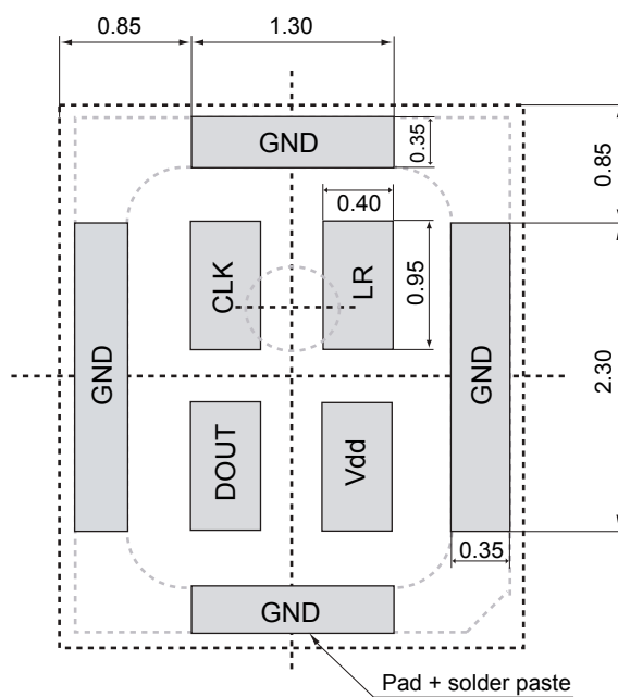
Figure 12. Land pattern
