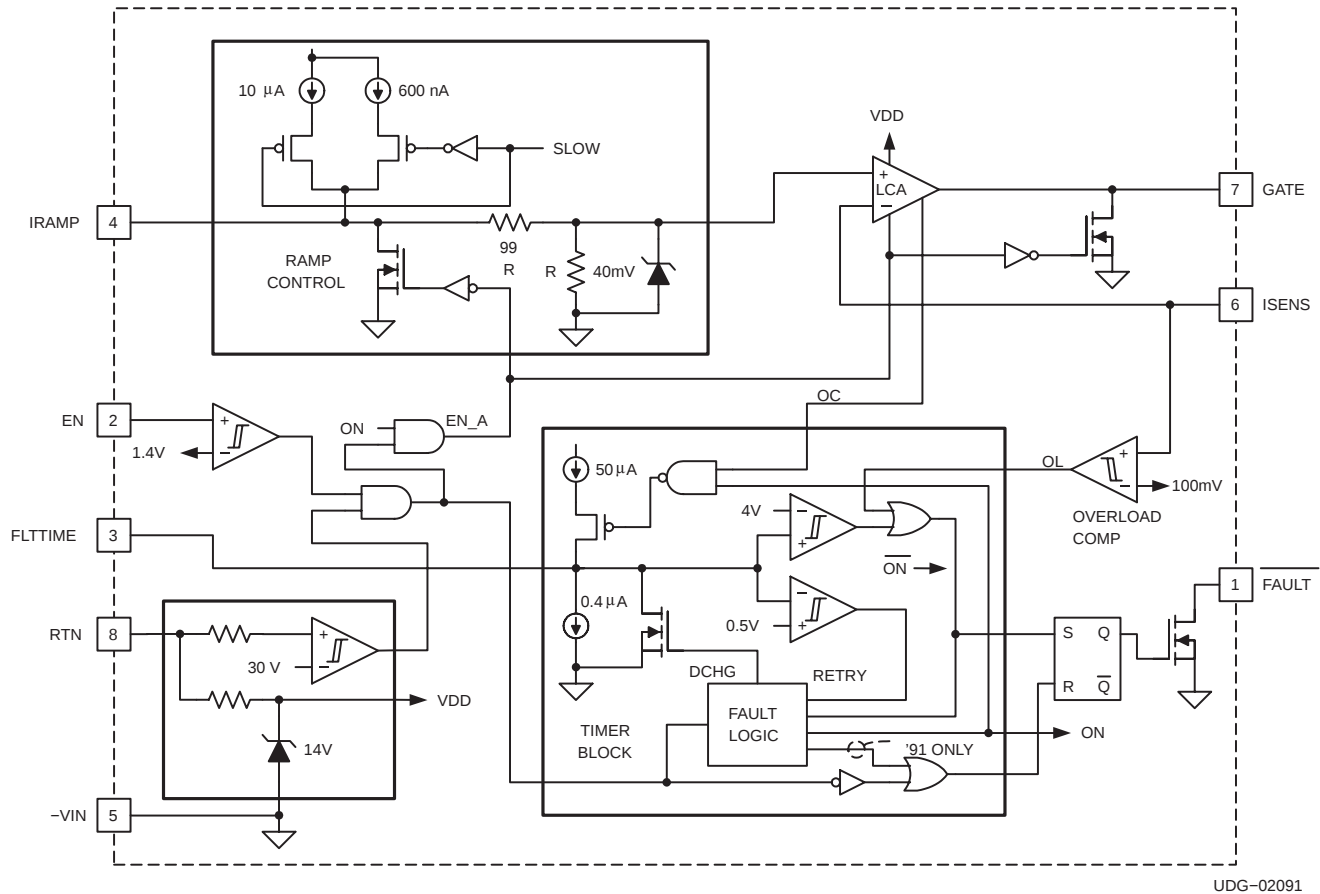
Figure 17. Block Diagram
