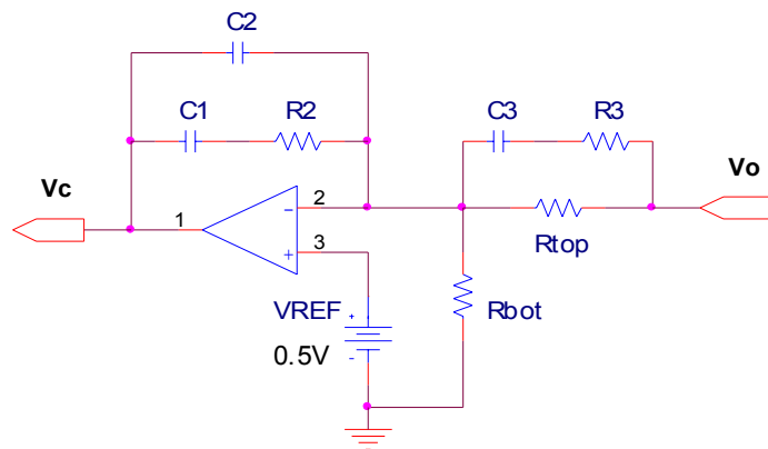
Fig. 5. Compensation network
