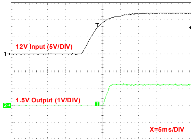
Transient Response
