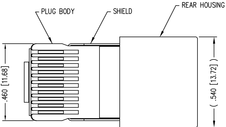
( SHOWN ASSEMBLED )
