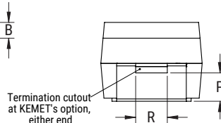
ANODE (+) END VIEW
