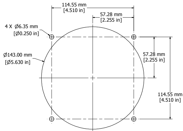
PLATE CUTOUT
