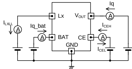
< Circuit No.④ >
