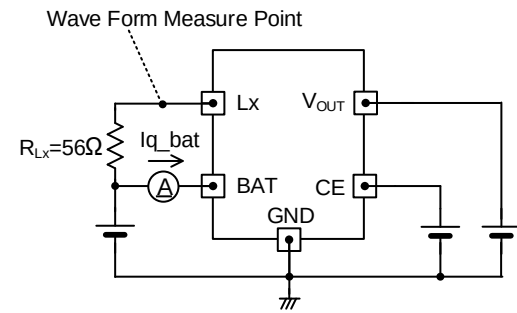
< Circuit No.④ >
