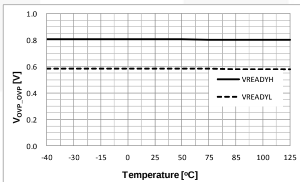
Figure 17. Ready Voltage vs. Temperature
