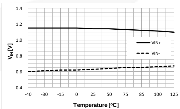
Figure 19. INPUT Threshold Voltage vs. Temperature
