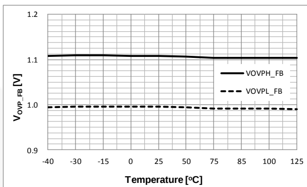
Figure 13. First OVP (FB) vs. Temperature
