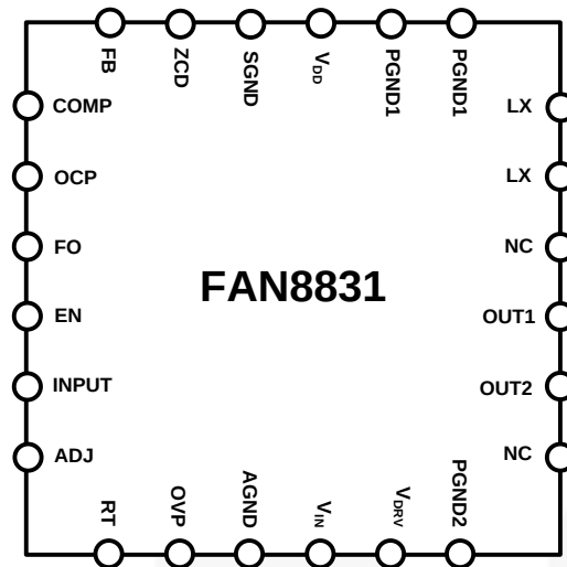
Figure 3. Pin Assignments
