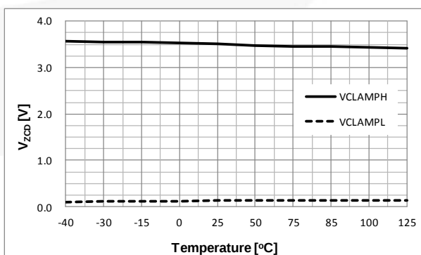
Figure 11. ZDC Clamp Voltage vs. Temperature
