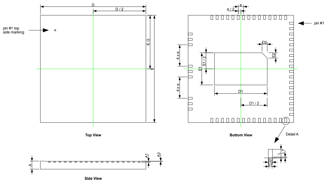
Figure 22-1. TQFN1010-57
