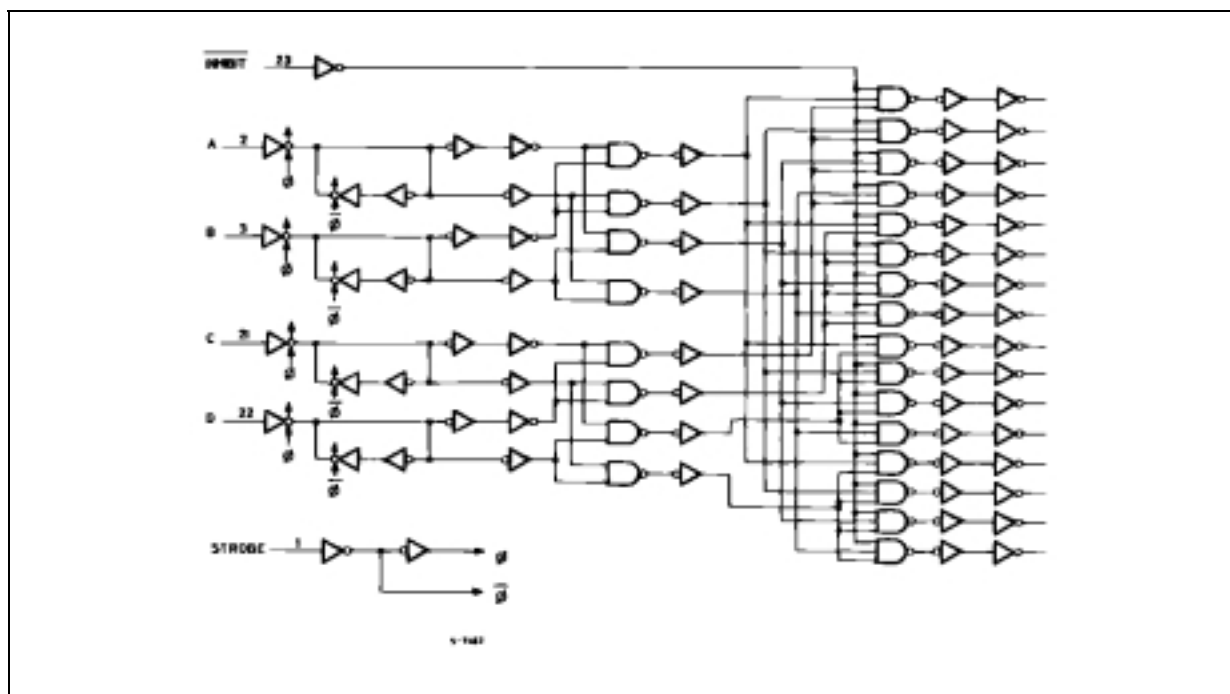
Figure 3: Logic Diagram
