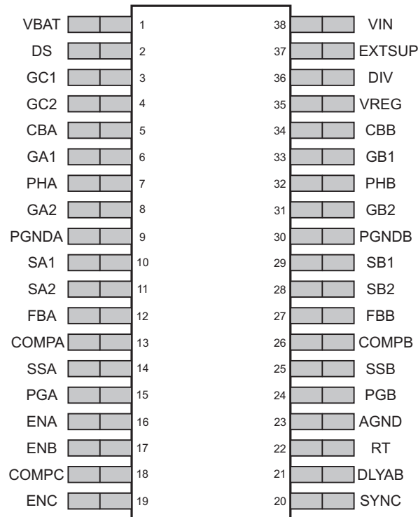
Pin Functions
