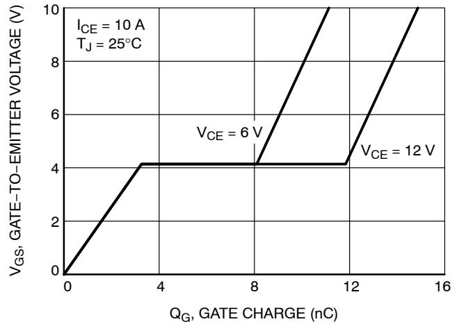
Figure 10. Gate Charge
