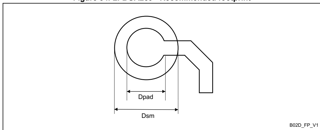
Figure 54. LFBGA289 - Recommended footprint
