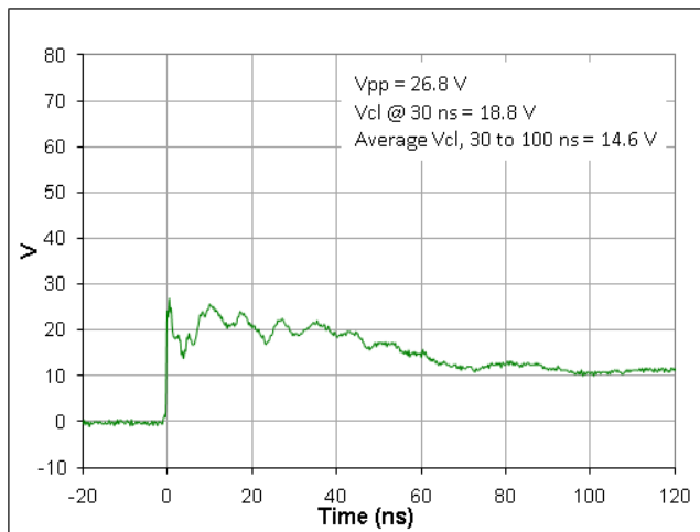
Figure 7. ESD Clamping Voltage Screenshot Positive 8 kV Contact per IEC61000-4-2, SDA line
