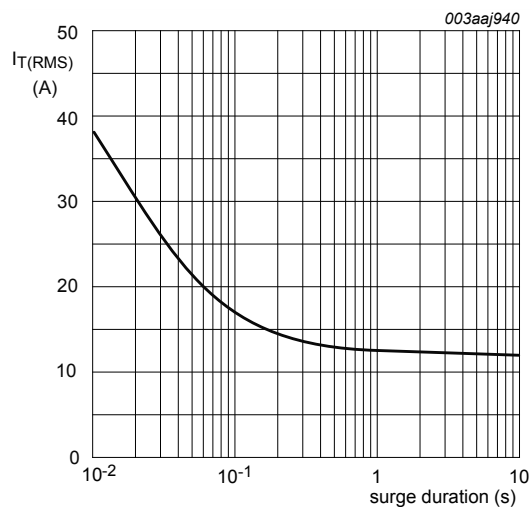
Fig. 2. RMS on-state current as a function of surge duration; maximum values f = 50 \text{ Hz}; T_{mb} = 99 \text{ °C}
