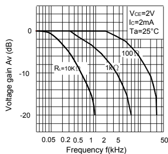
Fig. 10 Frequency Response
