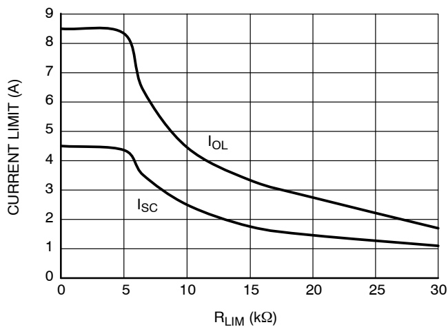
Figure 14. Overload and Short Circuit Current Limit vs R_{\text{LIM}}
