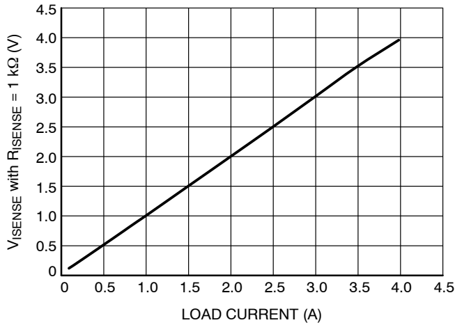
Figure 10. V_{\text{SENSE}} vs. Load Current
