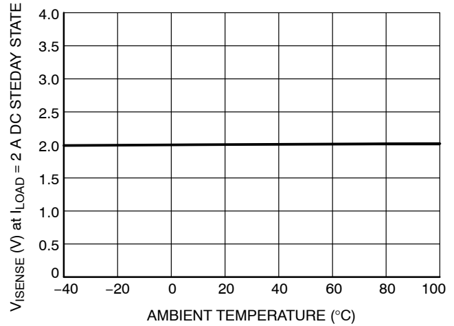
Figure 11. V_{\text{SENSE}} vs. Ambient Temperature
