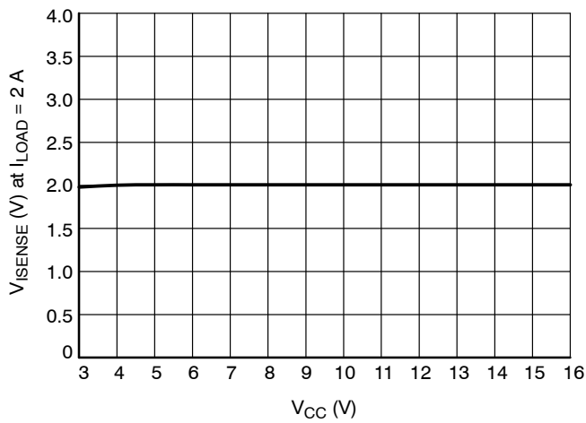
Figure 12. V_{\text{SENSE}} vs. V_{\text{CC}}
