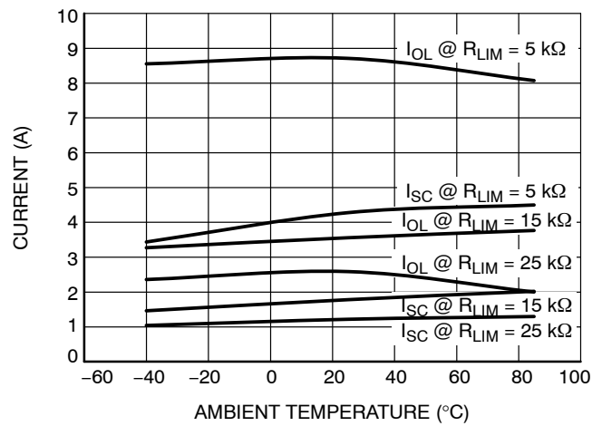
Figure 13. I_{\text{LIM}} vs. R_{\text{LIM}} over Ambient Temperature
