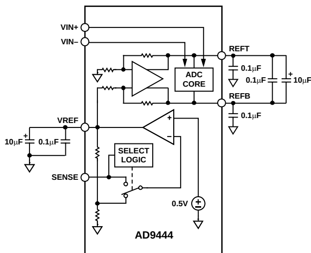
Figure 40. Internal Reference Configuration
