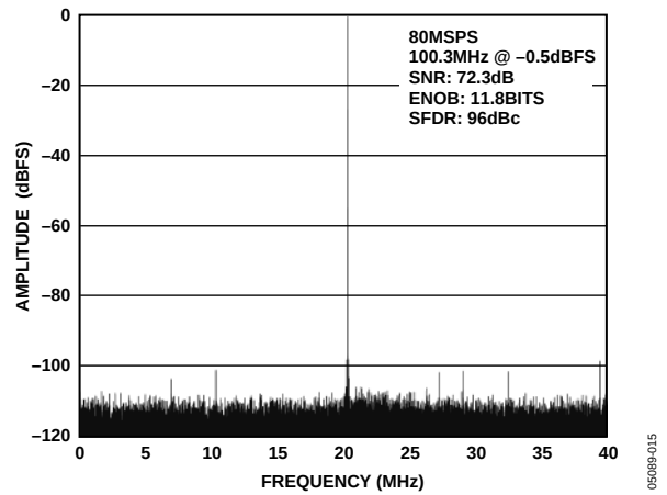
Figure 15. 64K Point Single-Tone FFT/80 MSPS/100 MHz
