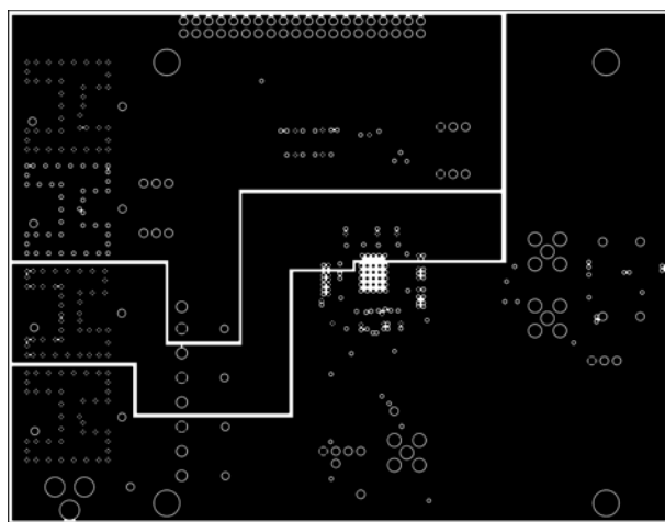
Figure 66. CMOS Mode Evaluation Board Layout, Power Plane 1
