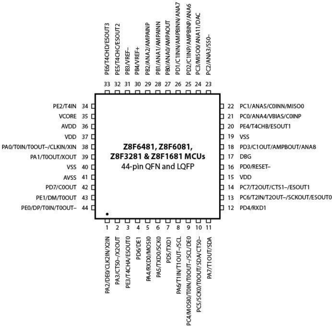
Z8Fxx81 MCUs: 44-Pin QFN and LQFP Configuration
