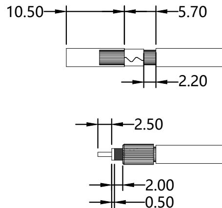
REFERENCE DIMENSION
