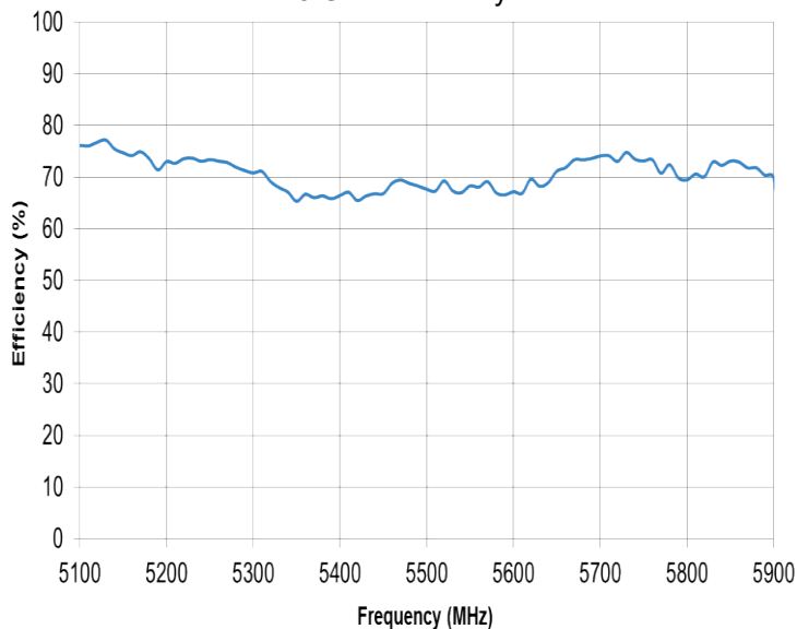
5 GHz Efficiency
