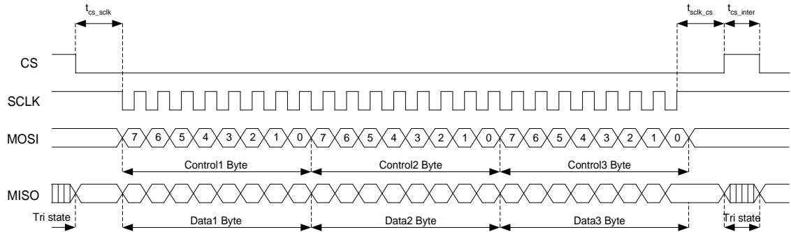
Figure 9 : SPI Timing Diagram for 3 byte instructions
