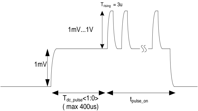
Figure 6: Vshunt waveform
