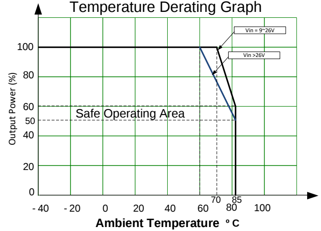
48Vin, 12/15/24Vout models Temperature Derating Graph
