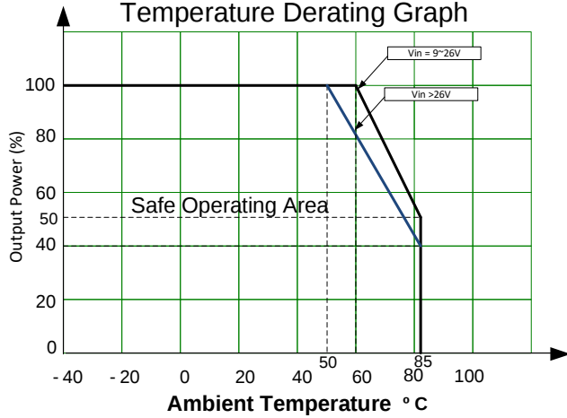
48Vin, 3.3/5Vout models Temperature Derating Graph
