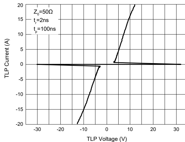
Fig. 4 - TLP Measurement
