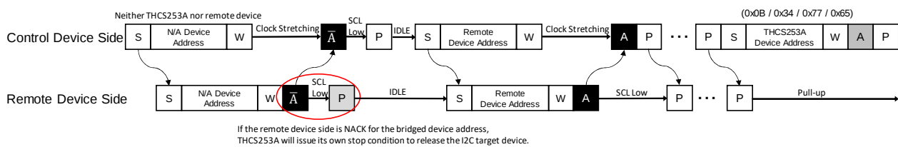
Figure 19 2-wire serial remote device access protocol (1)
