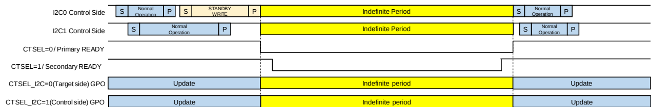
Figure 28 Normal => Standby (CTSEL_I2C=0/Primary , CTSEL_I2C=1/Secondary)
