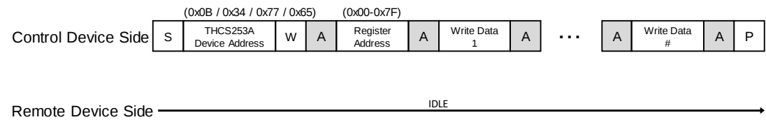
Figure 13 2-wire serial target register access protocol (1)
