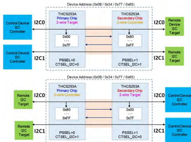
Figure 9 2-wire serial interface accessible range
