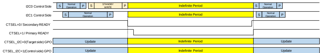
Figure 31 Standby => Normal (CTSEL_I2C=0/Secondary , CTSEL_I2C=1/Primary)
