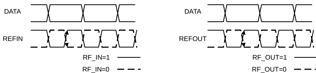
Figure 24 RF_IN, RF_OUT Function
