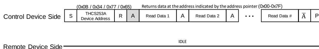
Figure 14 2-wire serial target register access protocol (2)
