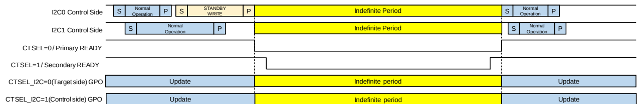
Figure 30 Standby => Normal (CTSEL_I2C=0/Primary , CTSEL_I2C=1/Secondary)
