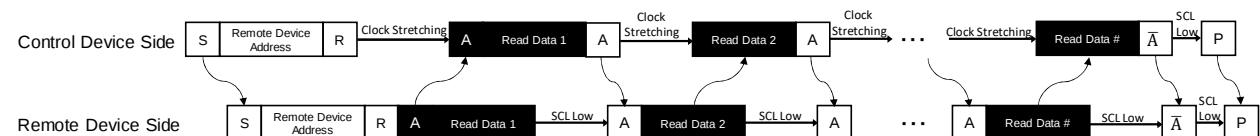
Figure 20 2-wire serial remote device access protocol (2)
