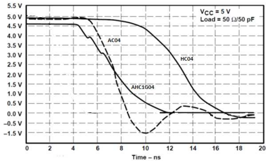
Figure 6. Typical Technology Output Drive Curve
