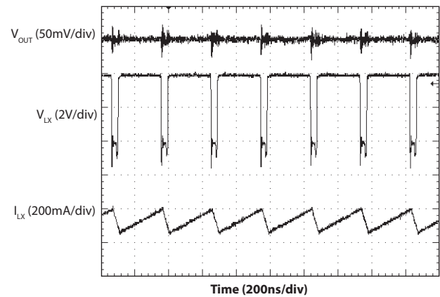
Heavy Load Switching — V_{OUT} = 3.3V
