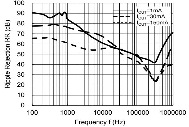
Ripple Rejection vs. Frequency AP7315Q-25
