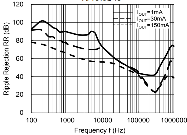
Ripple Rejection vs. Frequency AP7315Q-18
