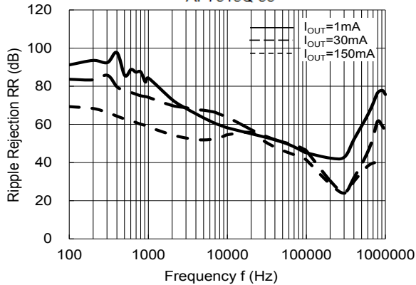
Ripple Rejection vs. Frequency AP7315Q-33
