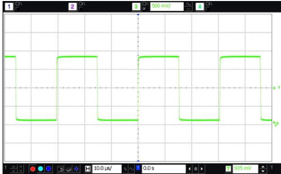
Figure 7. LVCMOS Waveform ( V_{dd} = 1.8\text{ V} ) into 15 pF Load
