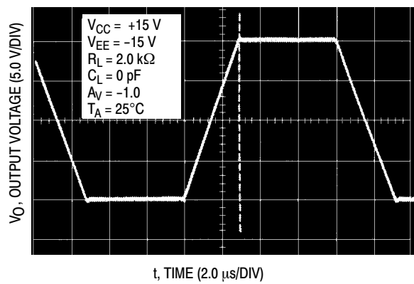
Figure 21. Inverting Amplifier
