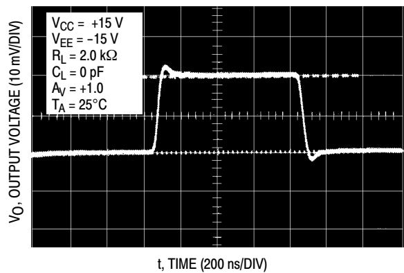
Figure 23. Noninverting Amplifier Overshoot
