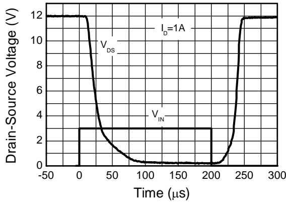
Switching Speed
