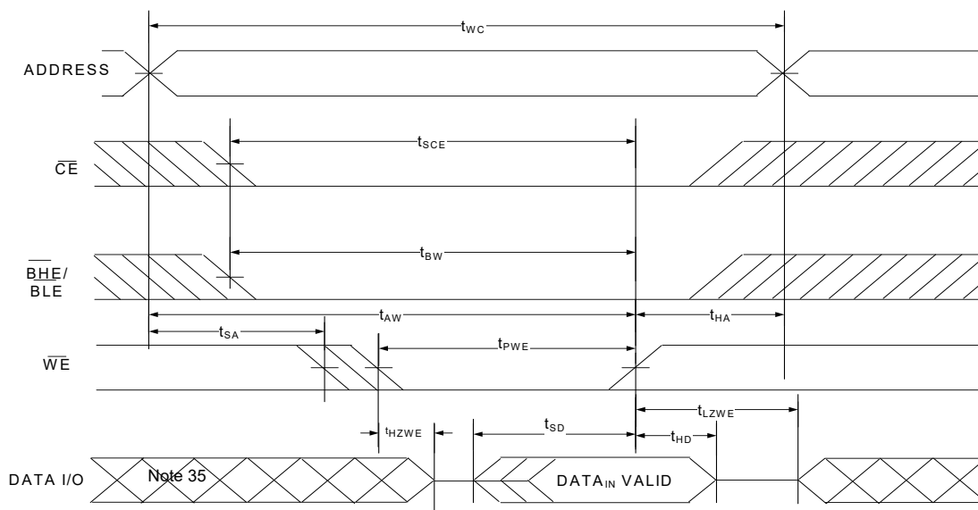
Figure 11. Write Cycle No. 1 ( \overline{\text{WE}} Controlled, \overline{\text{OE}} LOW) [31, 33, 34, 35]
