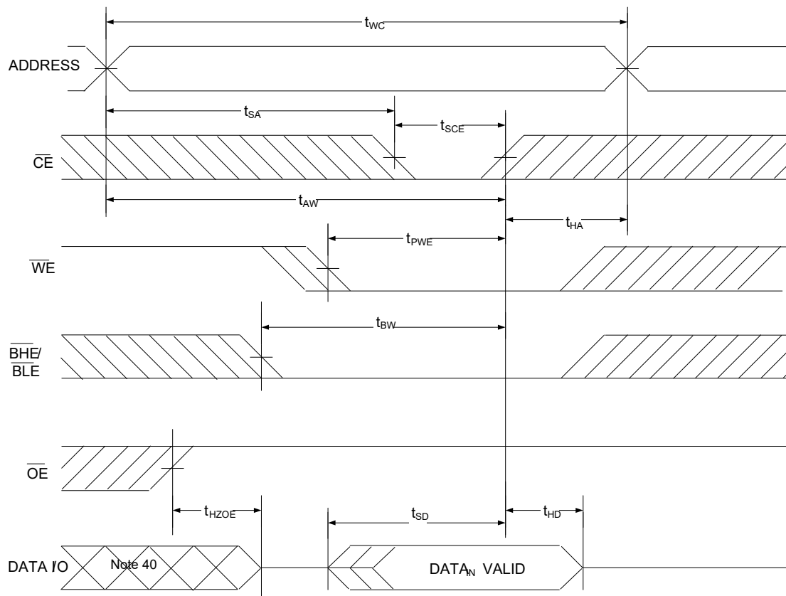
Figure 12. Write Cycle No. 2 ( \overline{\text{CE}} Controlled) [37, 38, 39]
