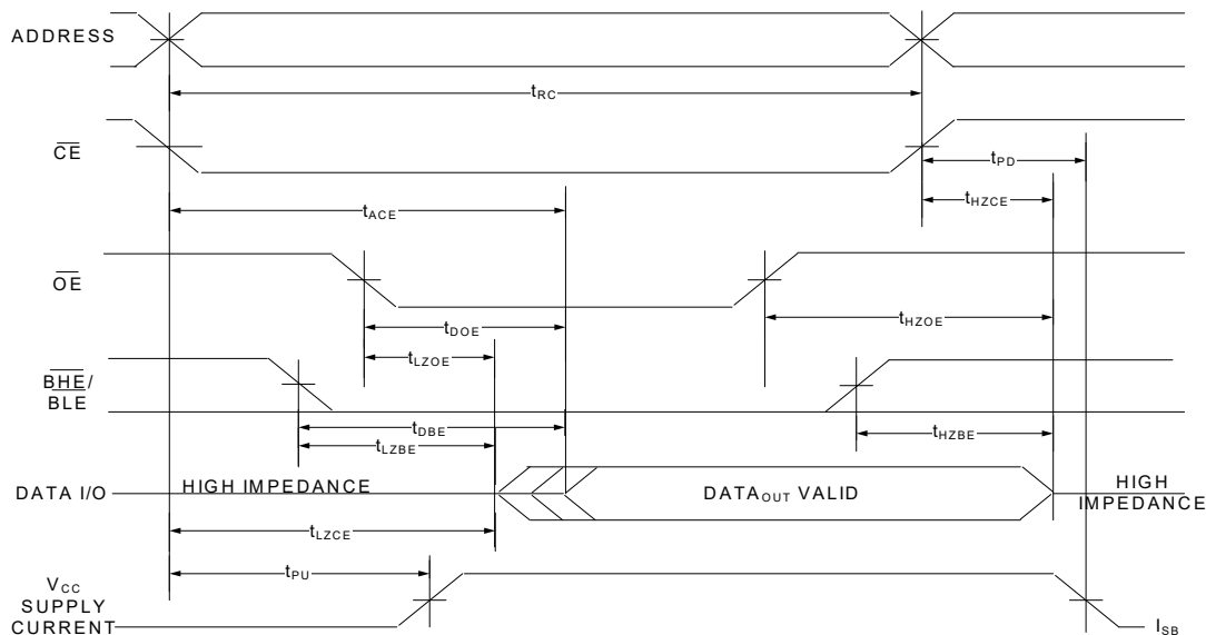
Figure 10. Read Cycle No. 2 ( \overline{\text{OE}} Controlled) [30, 31, 32, 34]
