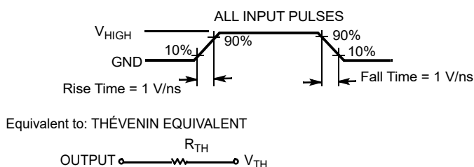
Figure 6. AC Test Loads and Waveforms
