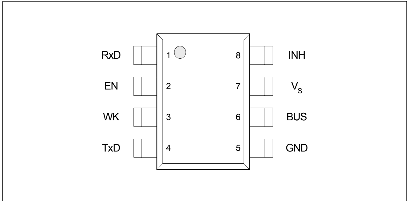
Figure 2 Pin Configuration
