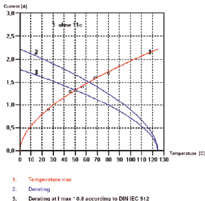
Derating curve
