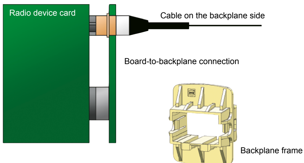
Fig. 4: Mini Coax backplane feed through
