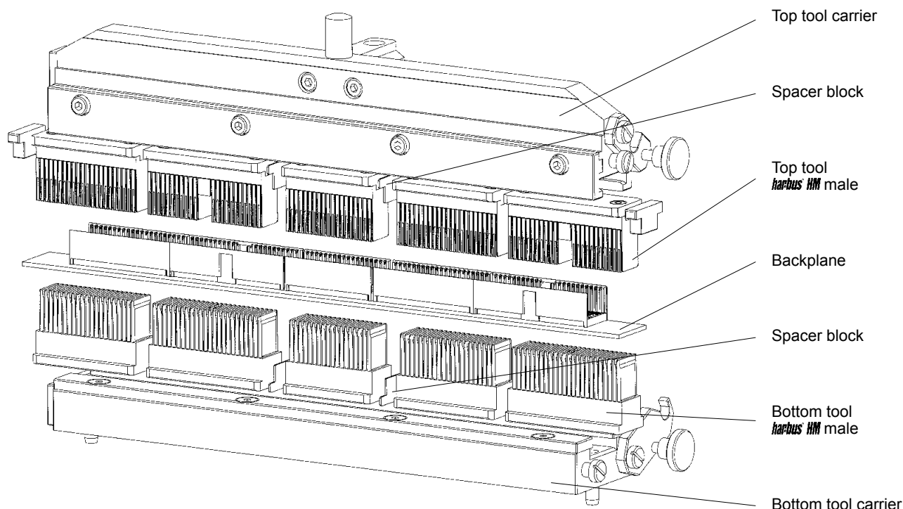
Fig. 2: Configuration sample for 6U backplane
