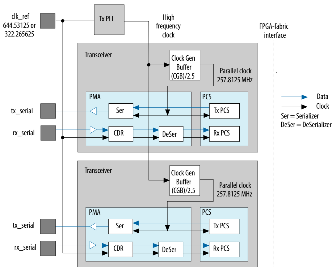
Provides a high-level view of the clock generation circuitry and clock distribution to the transceiver. In Sync-E variations, distinct clocks drive the TX PLL (tx_clk_ref) and the CDR block (rx_clk_ref), and the output clock from the CDR is brought out to the top level.
