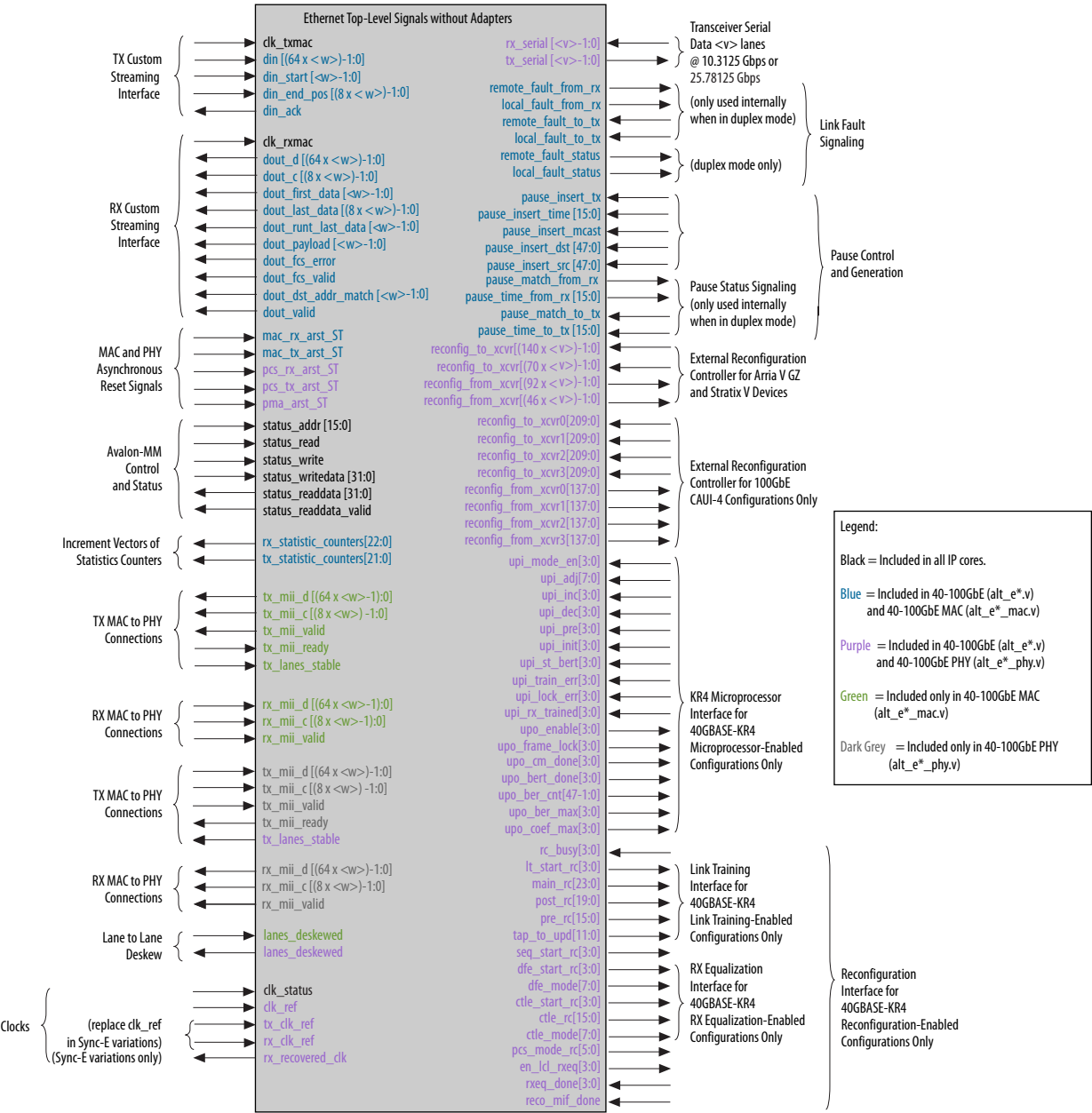
Figure 3-38: Top-Level Signals of the 40-100GbE IP Core Without Adapters
