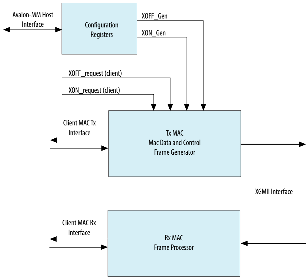
Figure 3-29: Block Diagram of the Pause Transmission Logic
