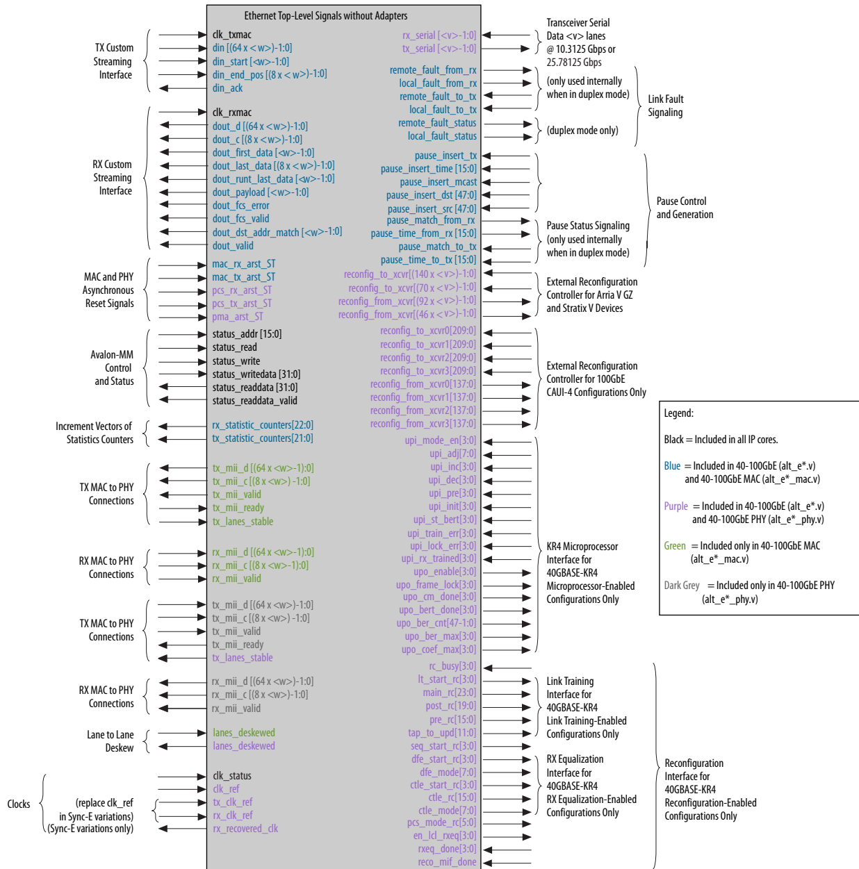
Figure 3-33: Top-Level Signals of the 40-100GbE IP Core Without Adapters
