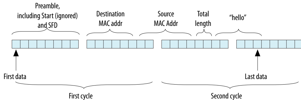
Example 3-2: Bus Representation of a Short TX Packet With Preamble
