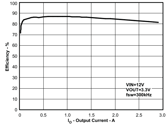
Figure 58. Efficiency vs Load Current
