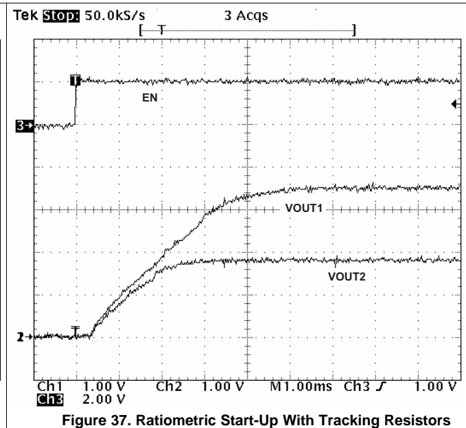
Figure 37. Ratiometric Start-Up With Tracking Resistors
