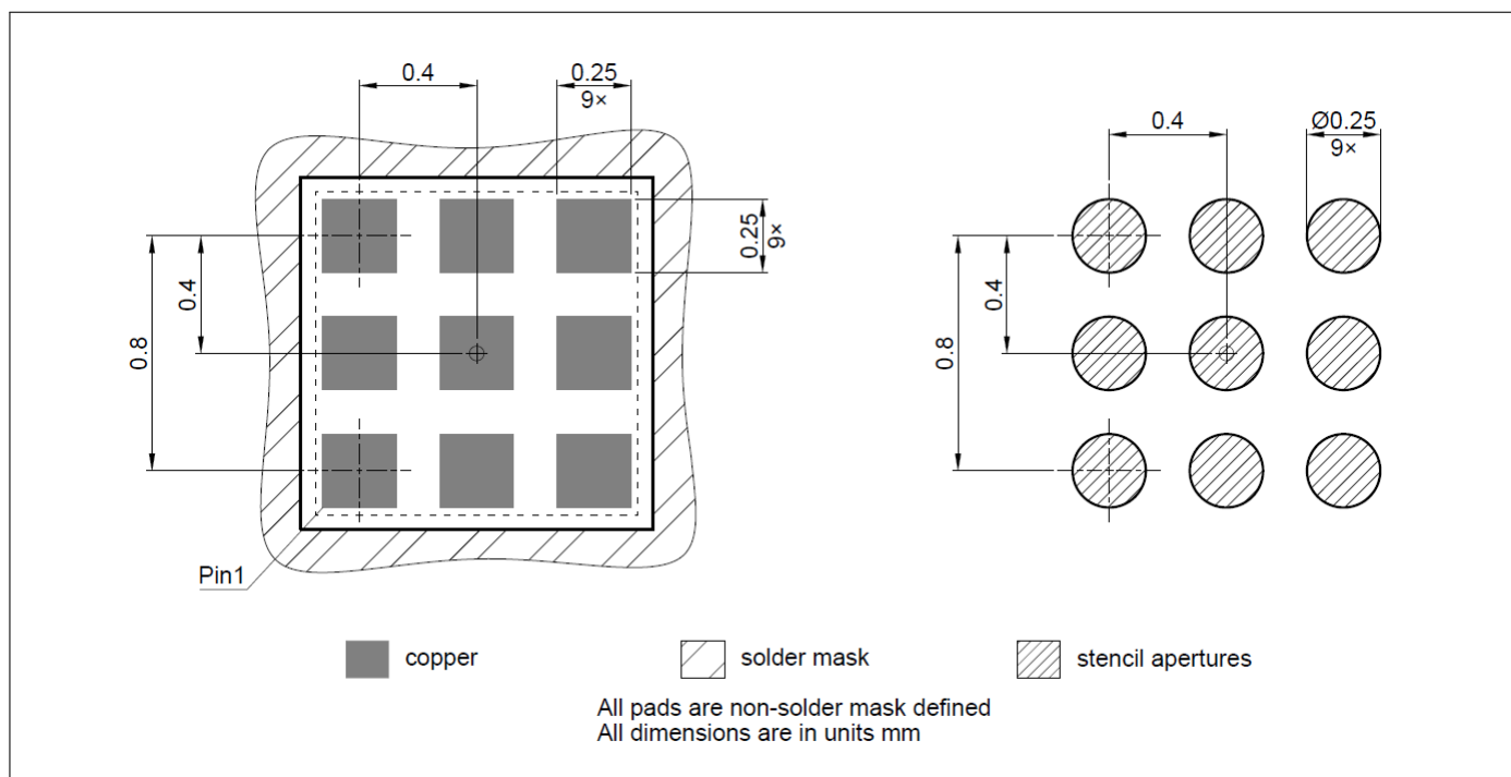
Figure 5: Footprint recommendation
