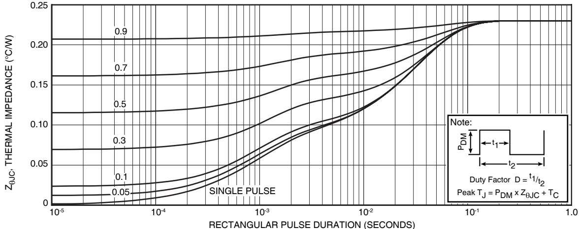
Figure 19, Maximum Effective Transient Thermal Impedance, Junction-To-Case vs Pulse Duration
