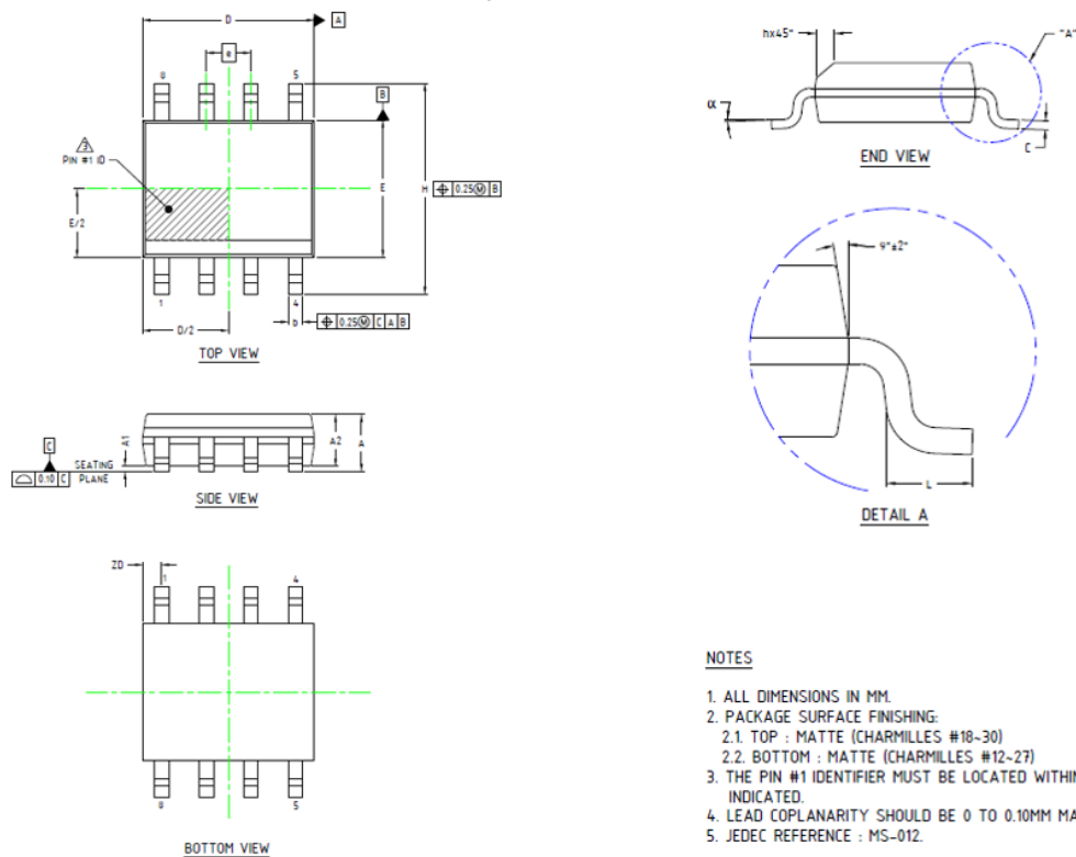
Figure 22: SOIC-8 Package Drawing and Dimensions
