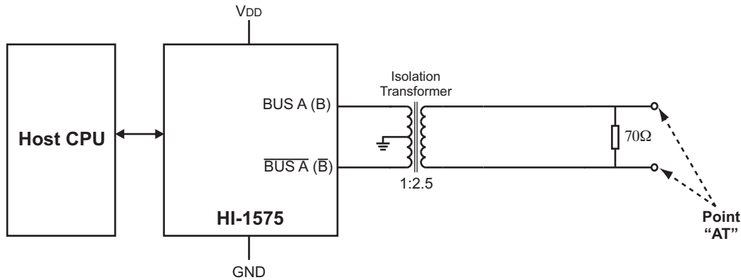
FIGURE 13. TRANSFORMER COUPLED TEST CIRCUIT
