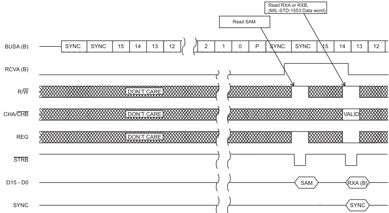
FIGURE 4. EXAMPLE RECEIVE OPERATION
