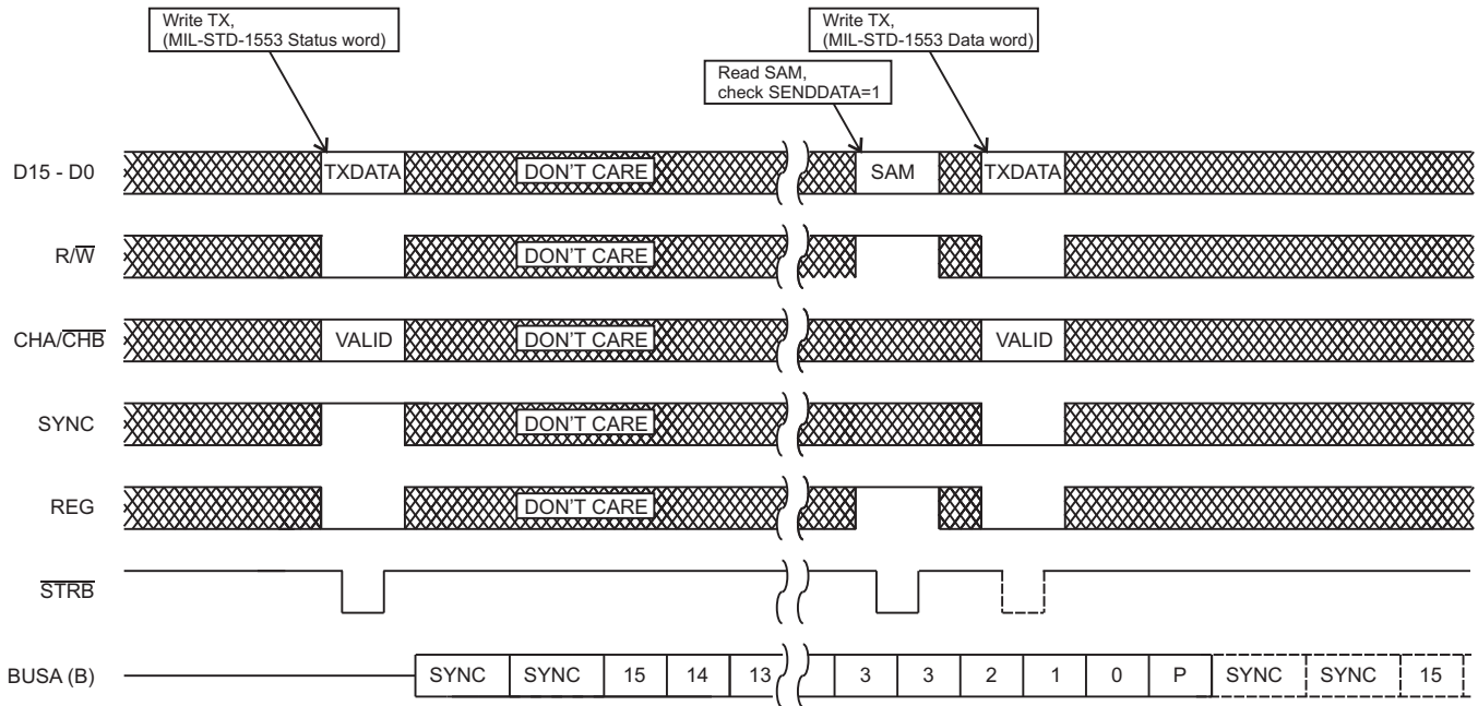
FIGURE 3. EXAMPLE TRANSMIT OPERATION
