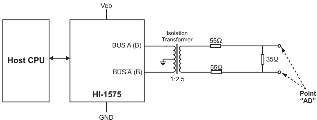
FIGURE 12. DIRECT COUPLED TEST CIRCUIT
