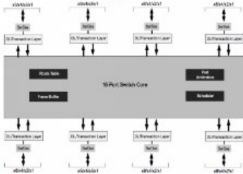
89H64H16AG2 - Block Diagram
