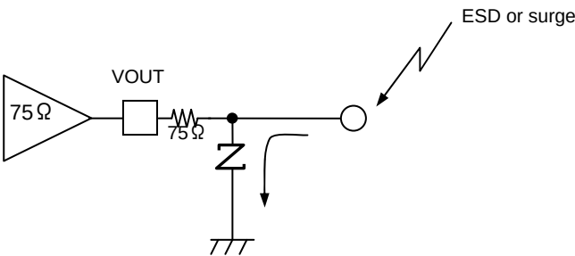
Fig.59 Using Externally Attached Varistor
