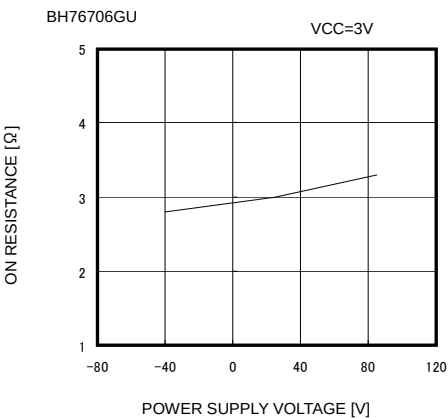
Fig. 58 Output Pin Shunt Switch On Resistance vs Ambient Temperature
