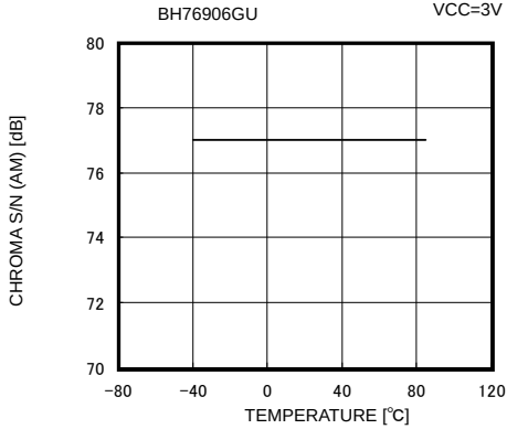
Fig. 50 C AM S/N vs Ambient Temperature
