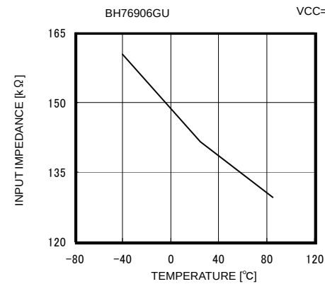
Fig. 54 Input Impedance vs Ambient Temperature
