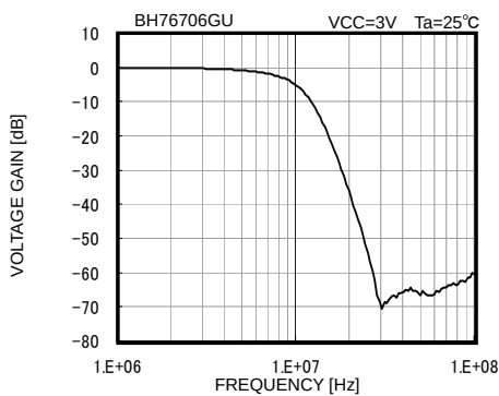
Fig. 25 Frequency Characteristic
