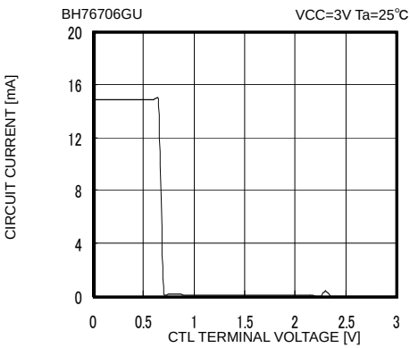
Fig. 56 Control Pin Characteristic
