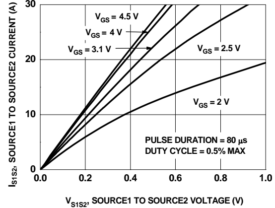
Figure 2. On-Region Characteristics
